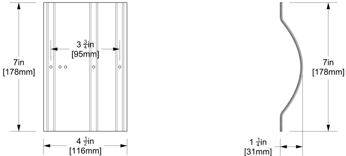
wall bracket
