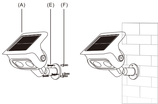
Wall mounted installation
