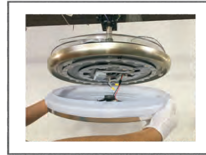
Step 4. Connect the Bluetooth drive cable on the lampshade with the Bluetooth cable on the chassis of the fan lamp host.
