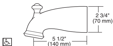
RP43165▲ (Non-Diverter)
