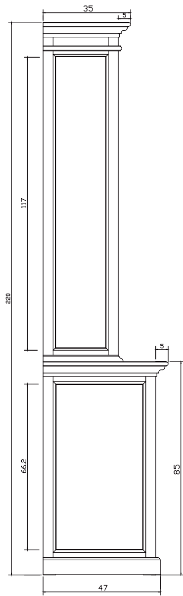
SIDE VIEW
