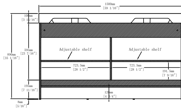
Back View
