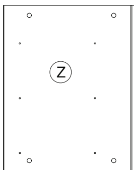
F17459 564x448x38mm
