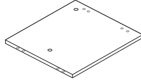
H-340x340x15mm(1pc)
