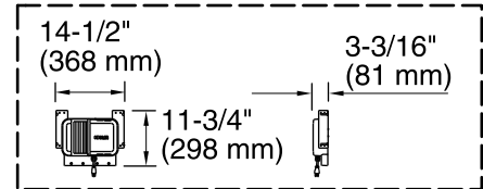
Control Amplifier
