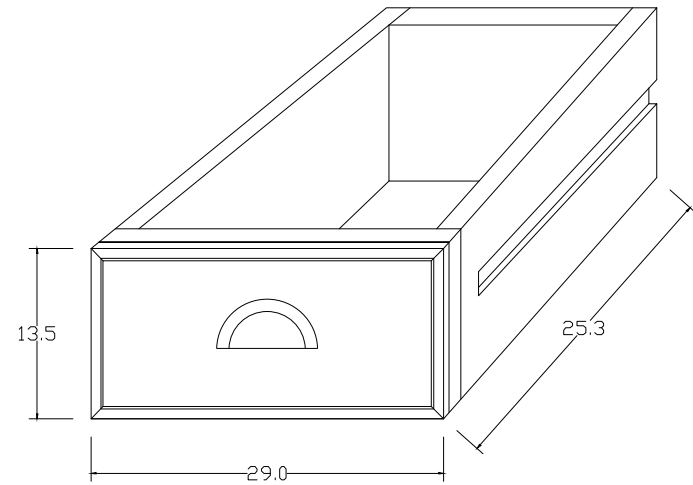
DETAIL DRAWER
