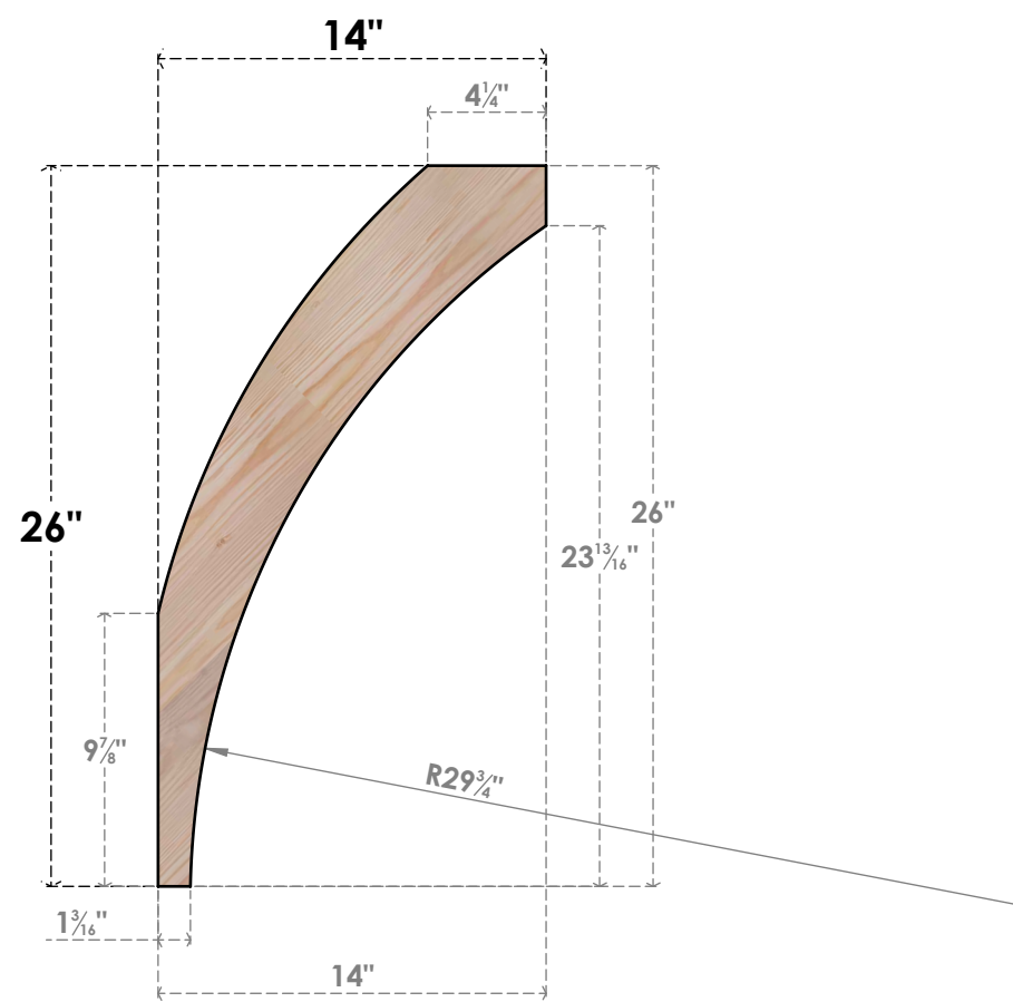
SIDE
