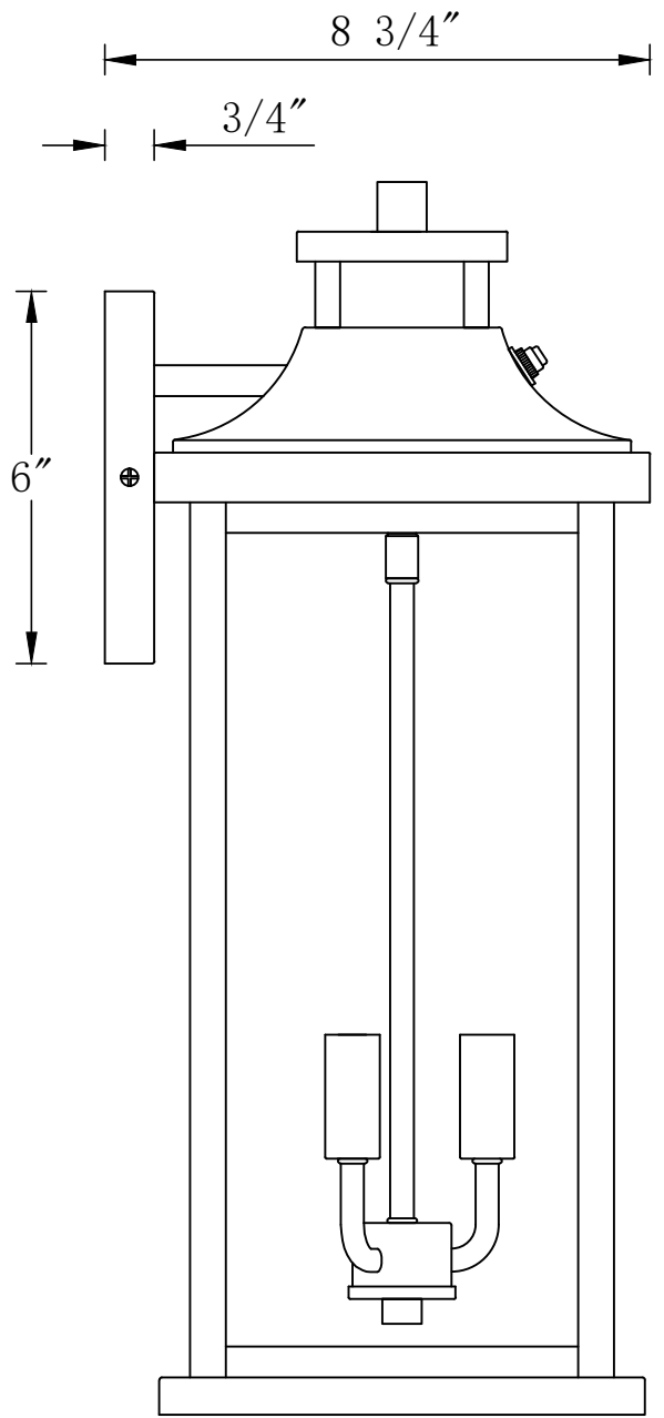
SIDE VIEW
