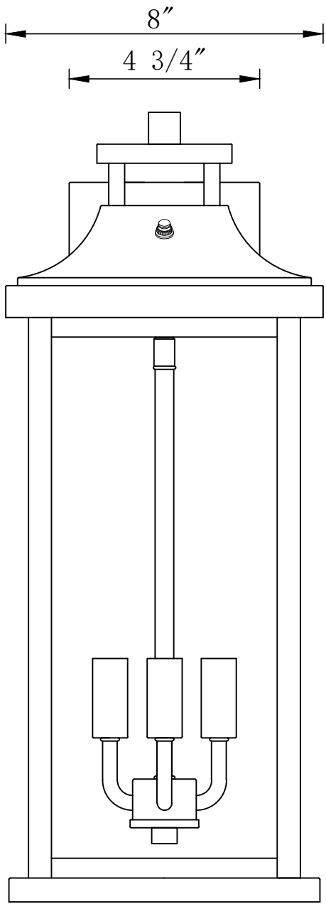
FRONT VIEW
