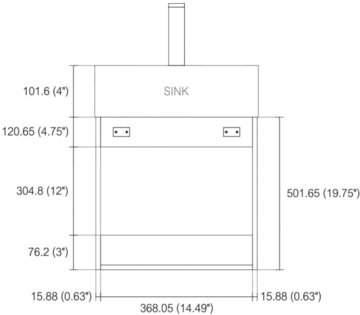
. BACK ELEVATION
