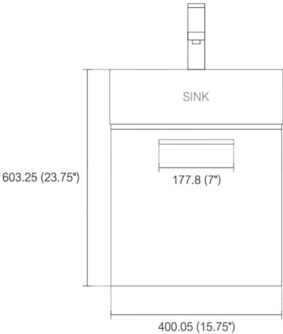
. FRONT ELEVATION
