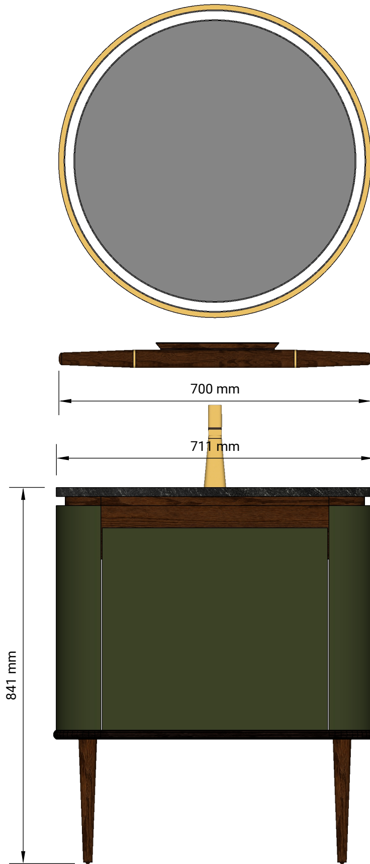
FRONT VIEW
