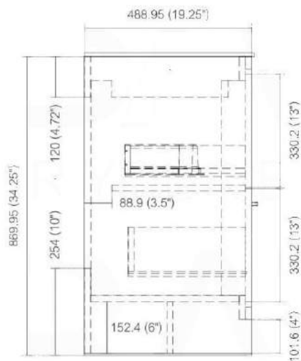
SIDE ELEVATION
