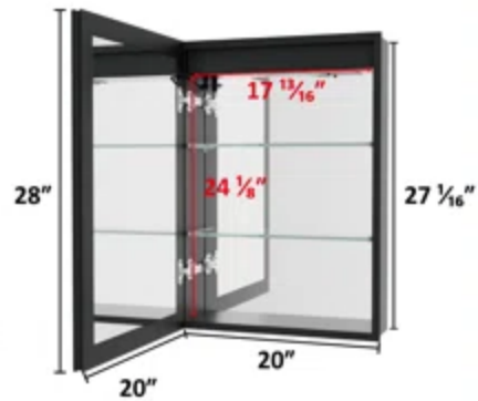
Cabinet Dimensions
