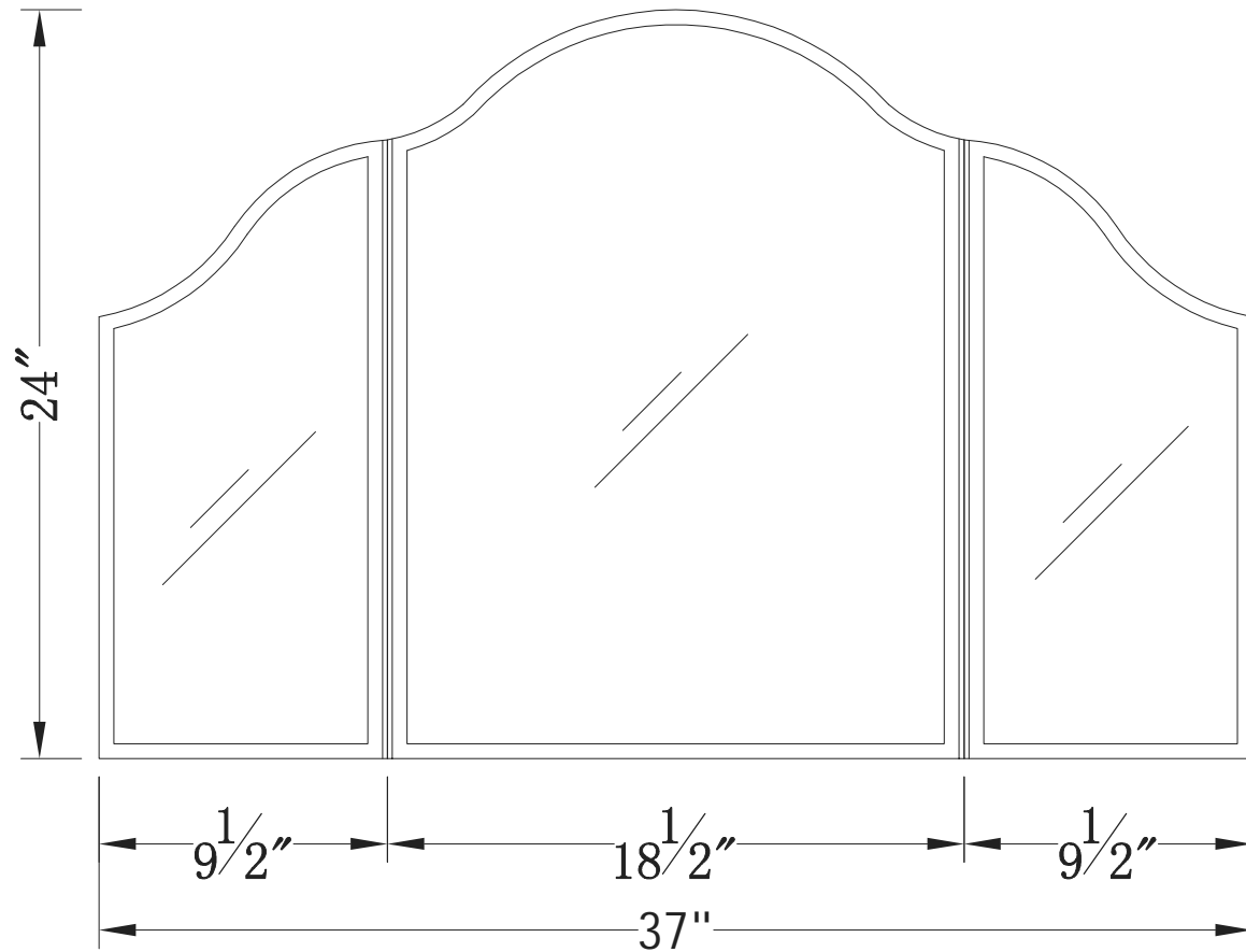
Front view
