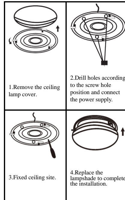
Installation method of circular ceiling lamp
