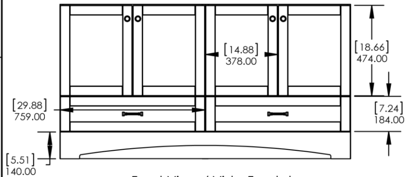
Front View / Vista Frontal
