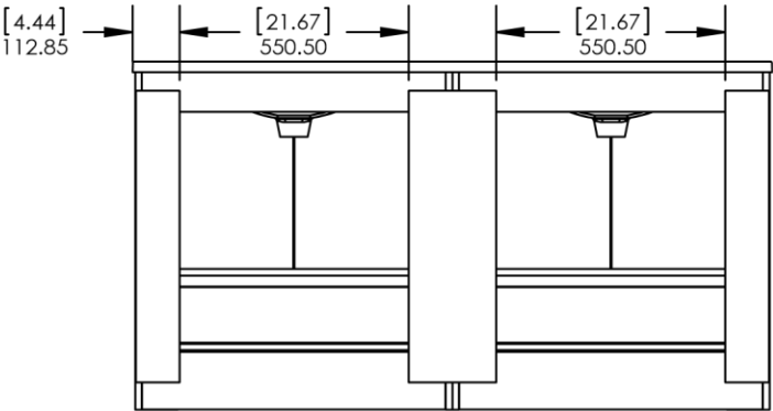
Back View / Vista Trasera
