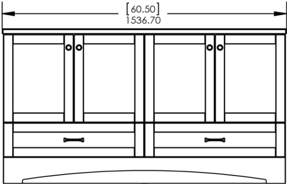
Front View / Vista Frontal
