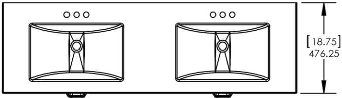
Top View / Vista Superior
