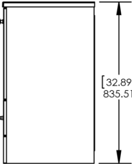
Side View / Vista Lateral
