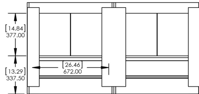
Back View / Vista Trasera
