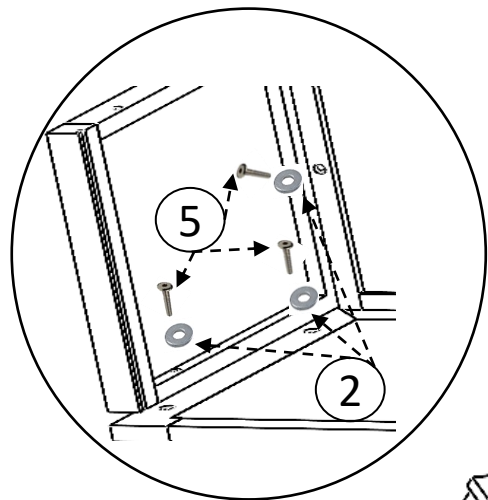
DETAIL Z
