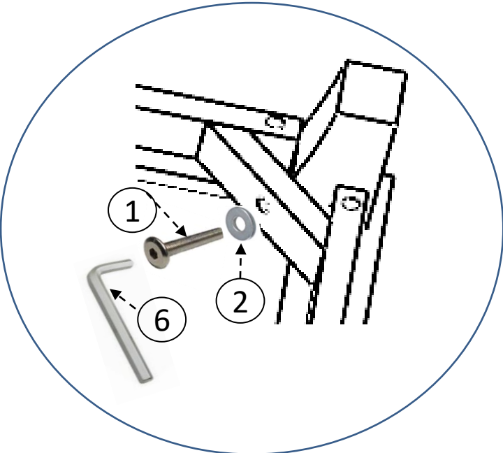
DETAIL X
