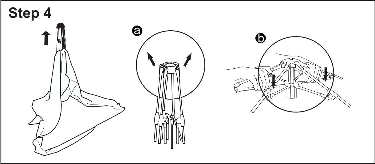
Hold the top of the tent and lift it up, and then press the top down to make sure that the tent is fully buckled
