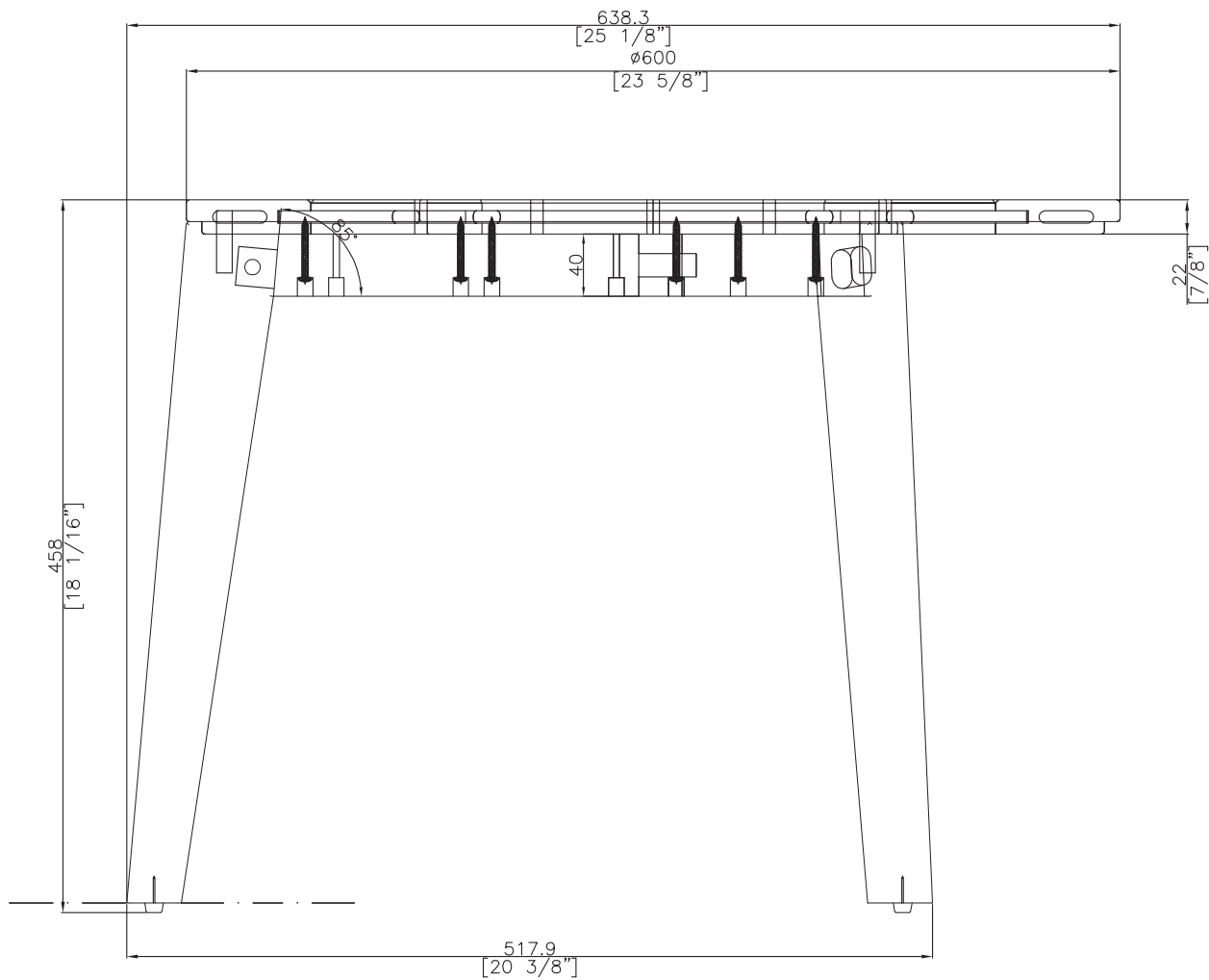
SIDE VIEW
