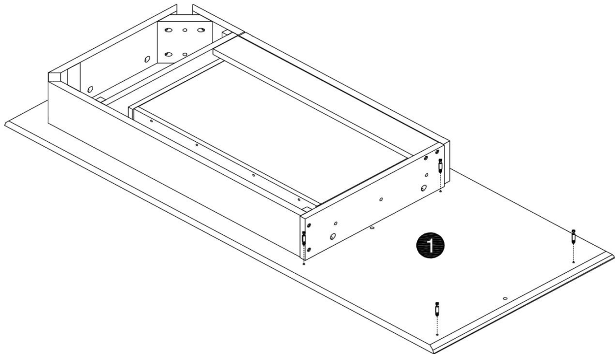
B.CAM SCREW - 4
