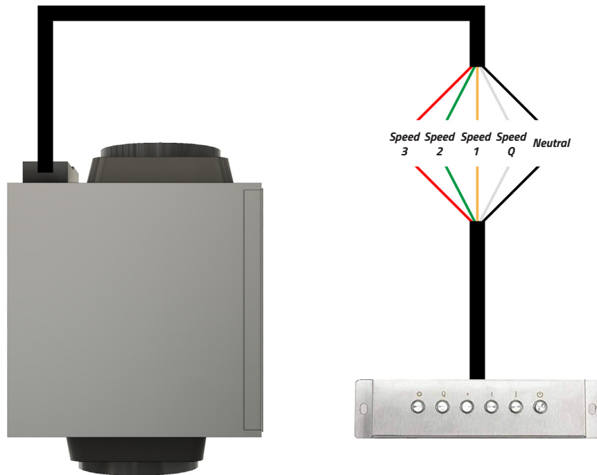
Connecting the Blower Unit to an Awoco Split Hood Unit or a Control Unit
