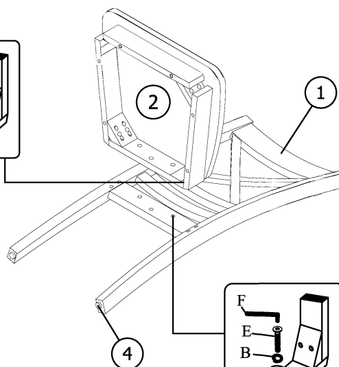
DETAIL B
