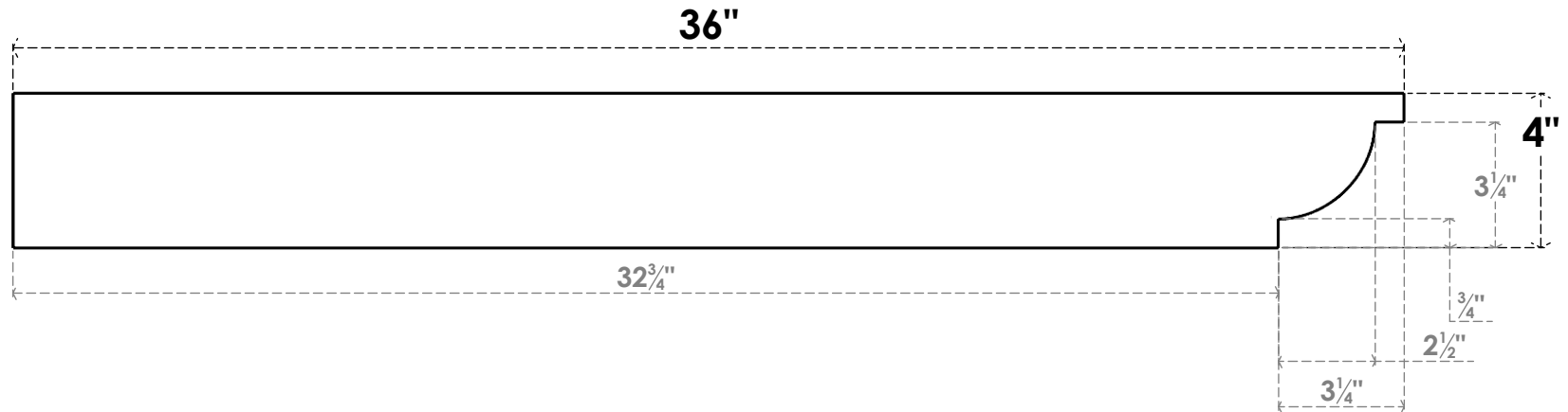
SIDE PROFILE
