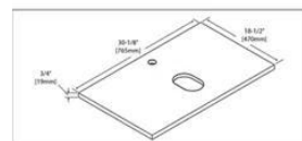
COUNTER-TOP
