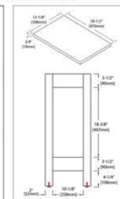
12" CABINET TOP&BACK
