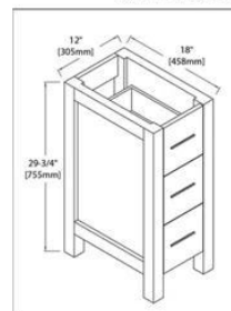
12" CABINET FRONT
