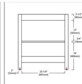
VANITY BACK
