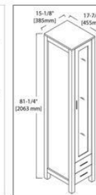
15" CBINET FRONT
