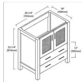
VANITY FRONT
