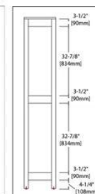
15" CBINET BACK
