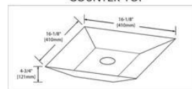
SINK
