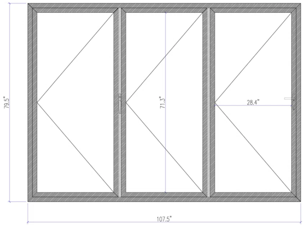
Front View Dimension
