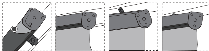
Fig 6-Wall Mount
