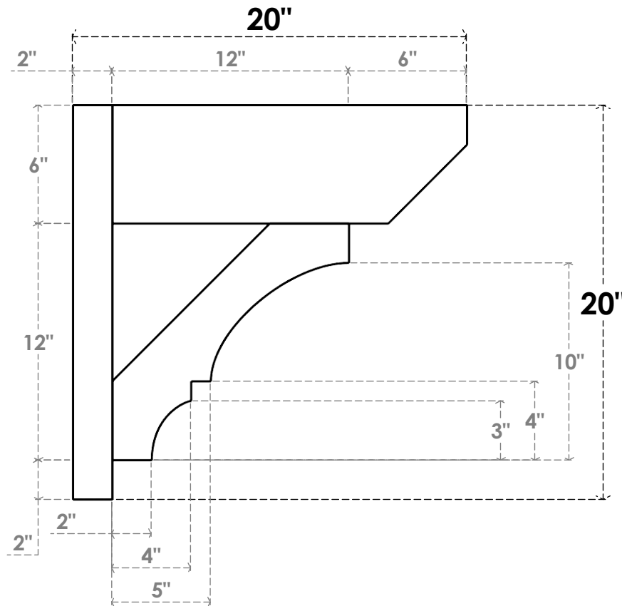
SIDE PROFILE
