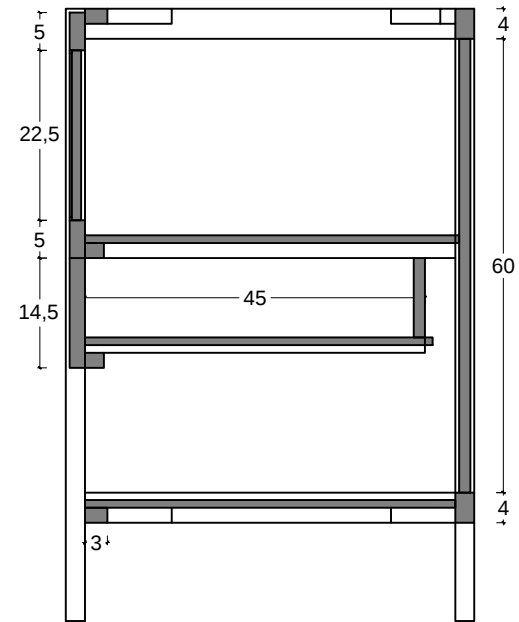
SIDE SECTION
