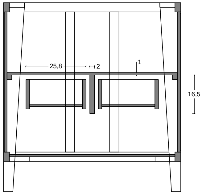
FRONT SECTION
