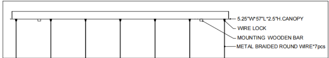
CANOPY DETAIL
