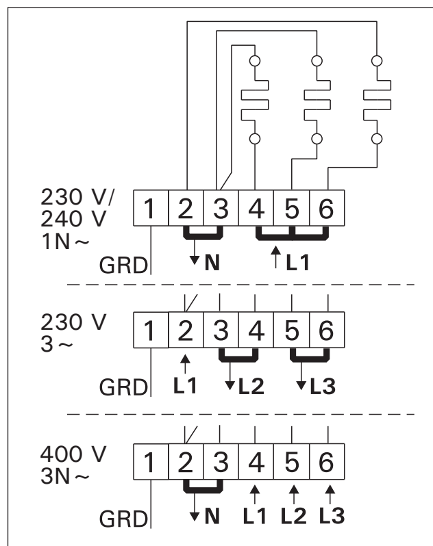
Figure 11. Electrical connections of BC-E heater Abbildung 11. Elektroanschlüsse des Saunaofens BC-E
