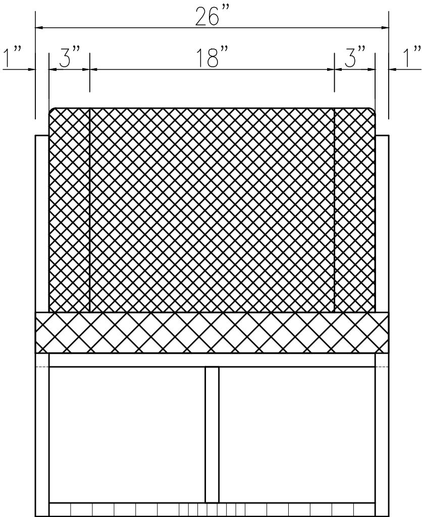
Front View
