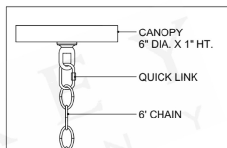
CANOPY DETAIL
