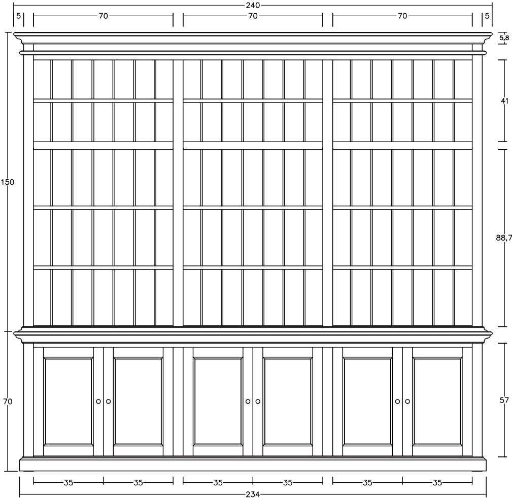
FRONT VIEW
