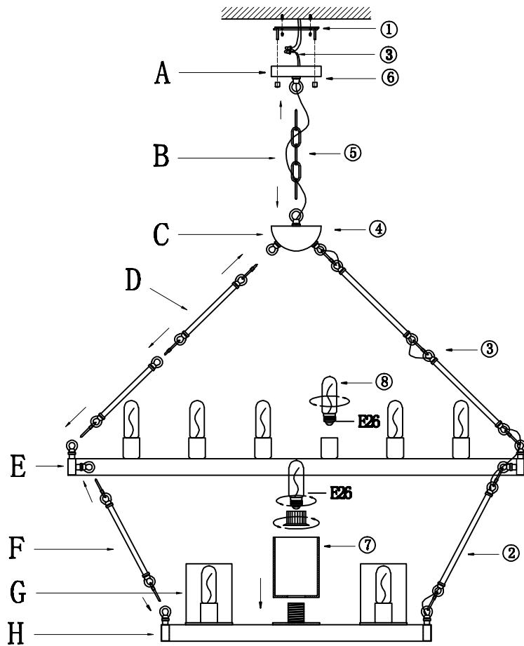
Installation sequence diagram
