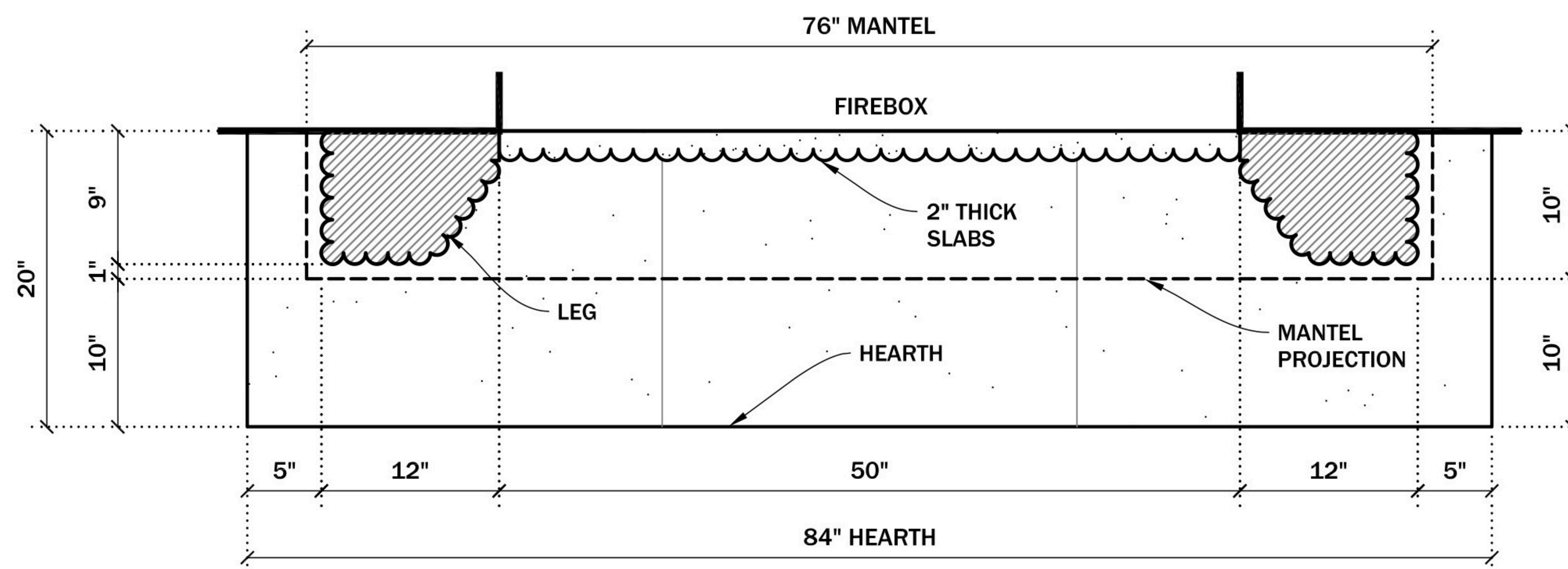
PLAN VIEW
