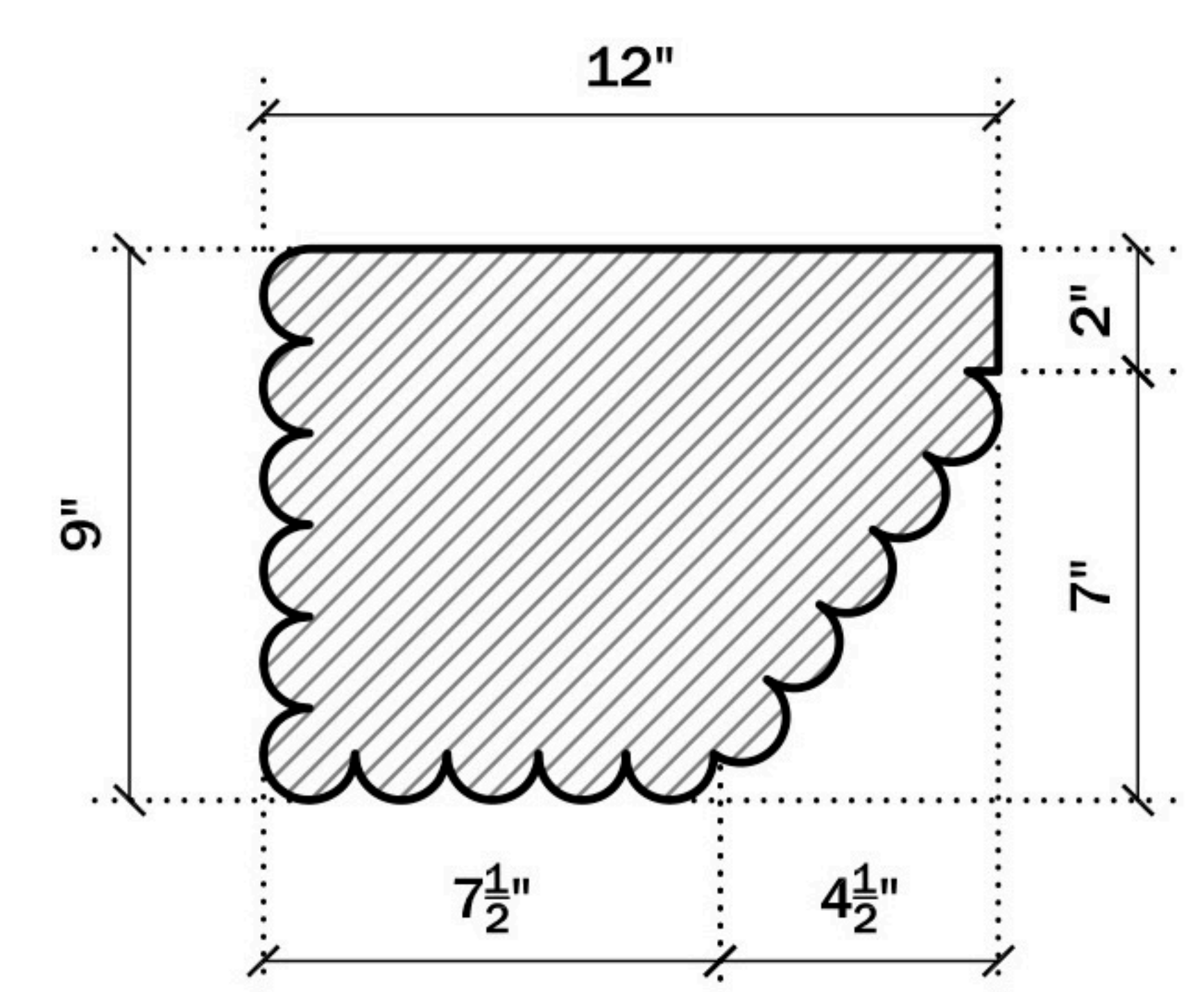
LEGS PROFILE
