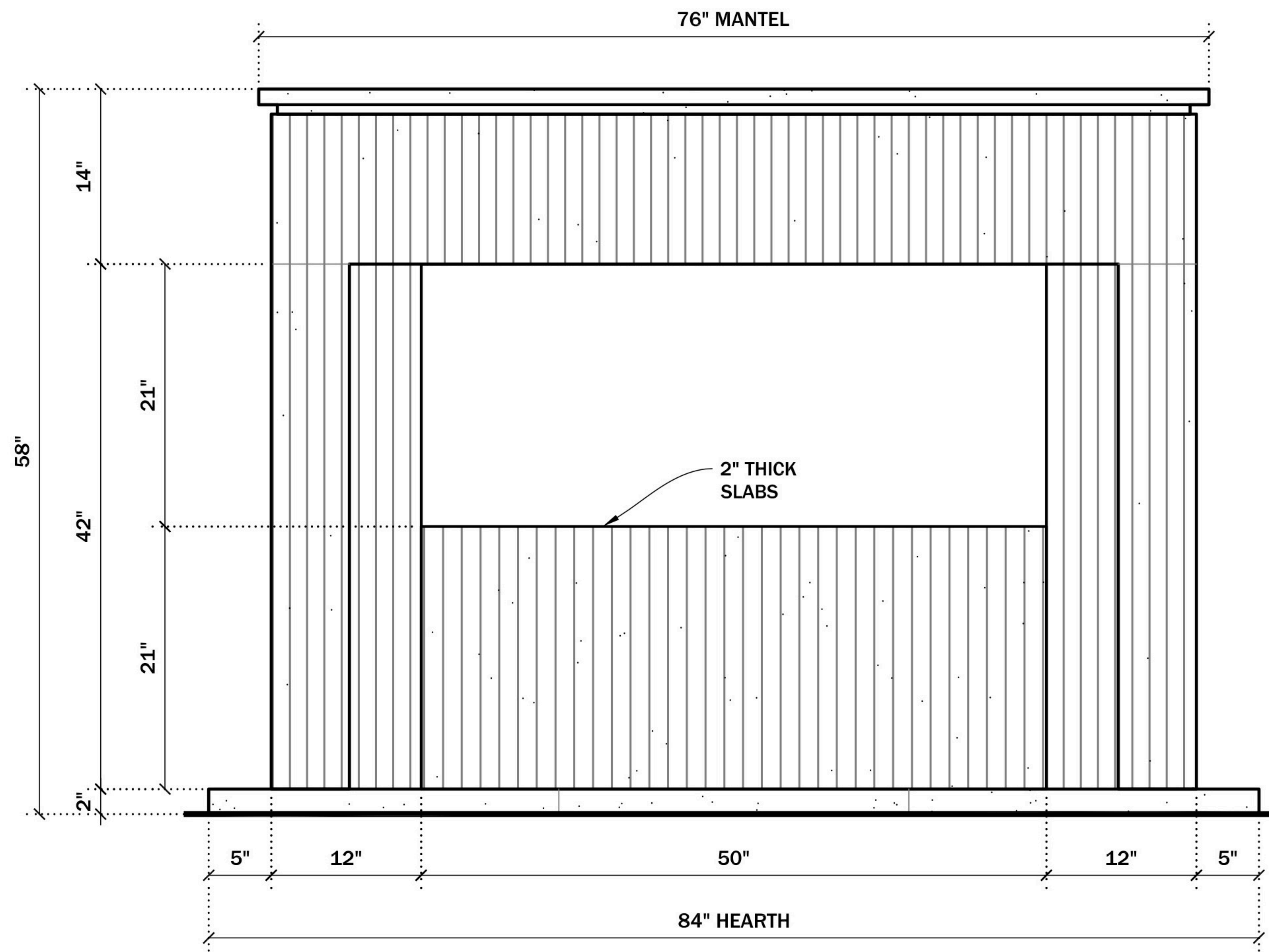
FRONT ELEVATION
