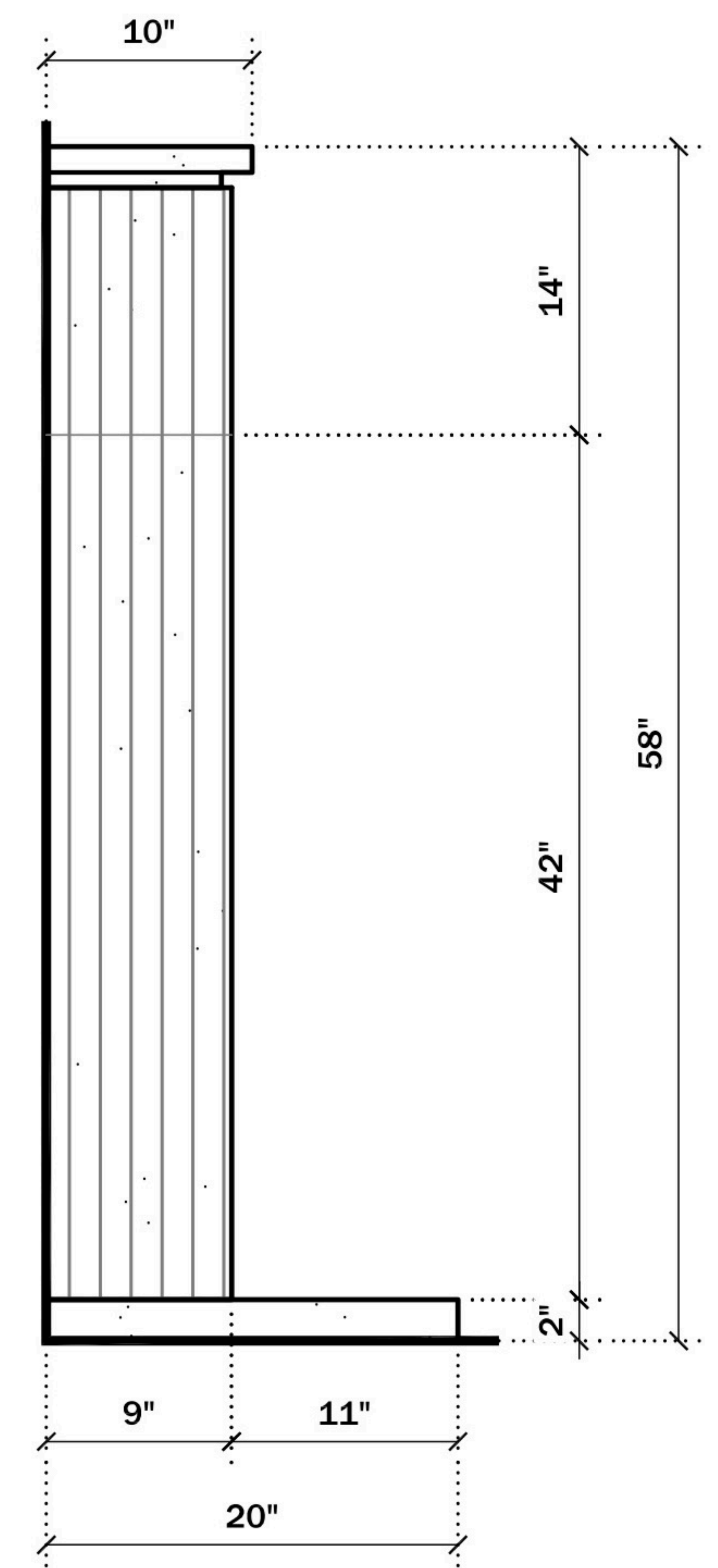
SIDE VIEW
