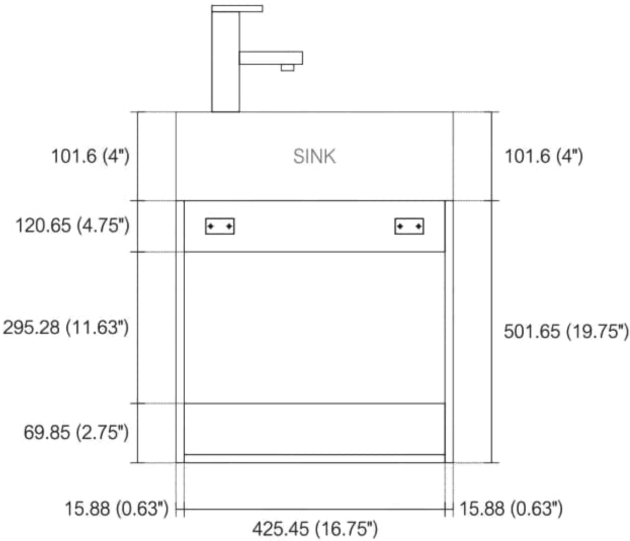
. BACK ELEVATION
