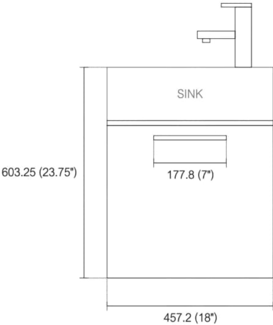
. FRONT ELEVATION
