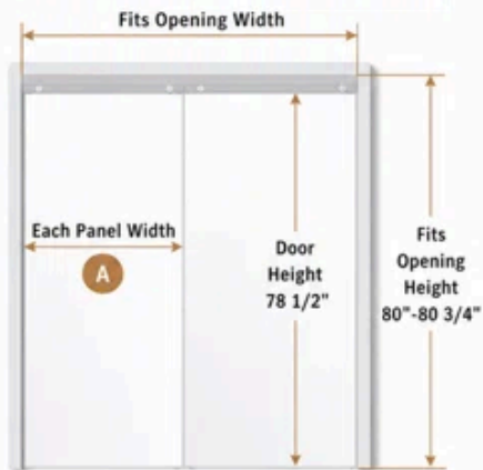
2 Panels Sliding Door (Single Opening)
