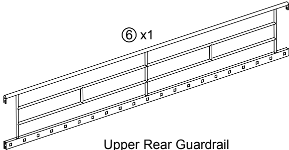
Upper Rear Guardrail
