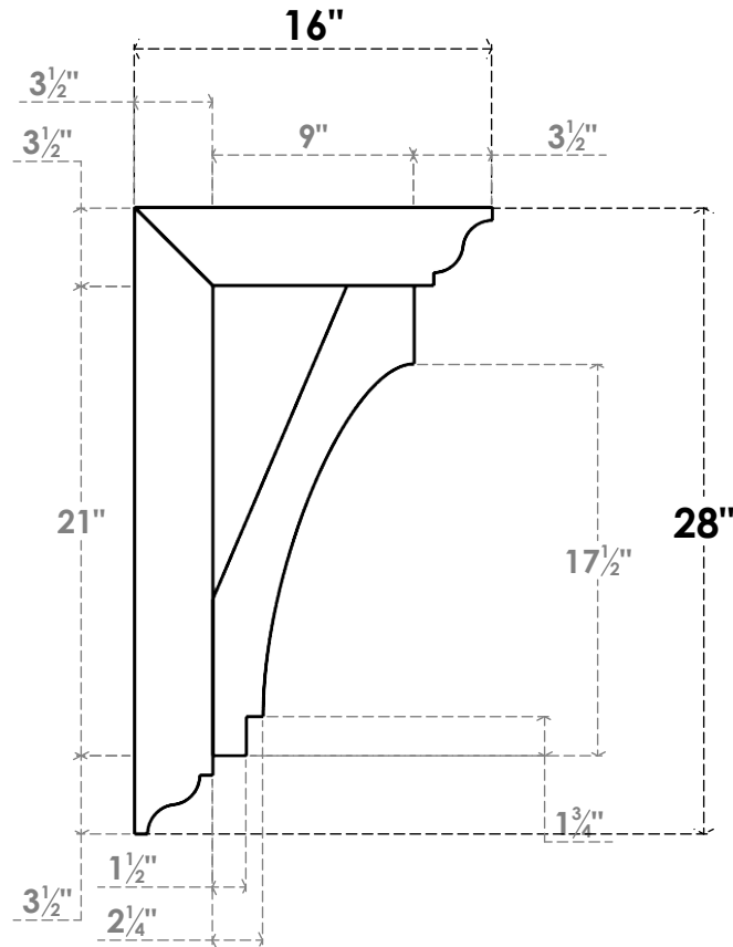
SIDE PROFILE
