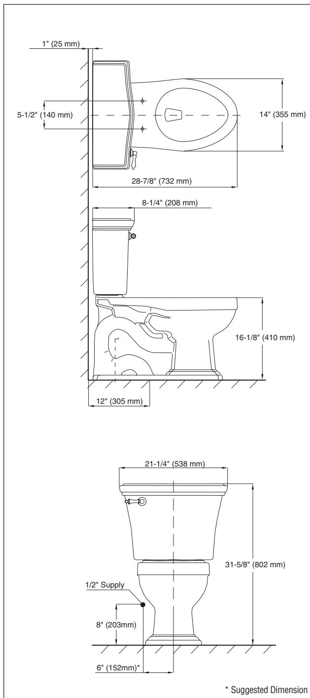
CST784SF - Clayton™ Toilet
