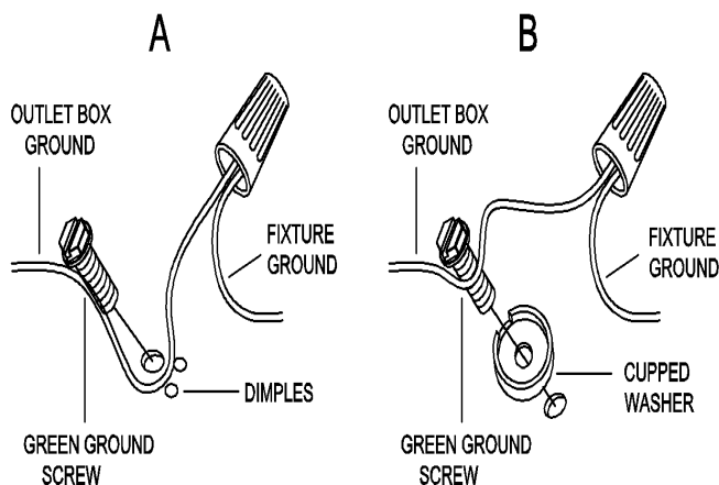
Connect ground wire according to below chart
