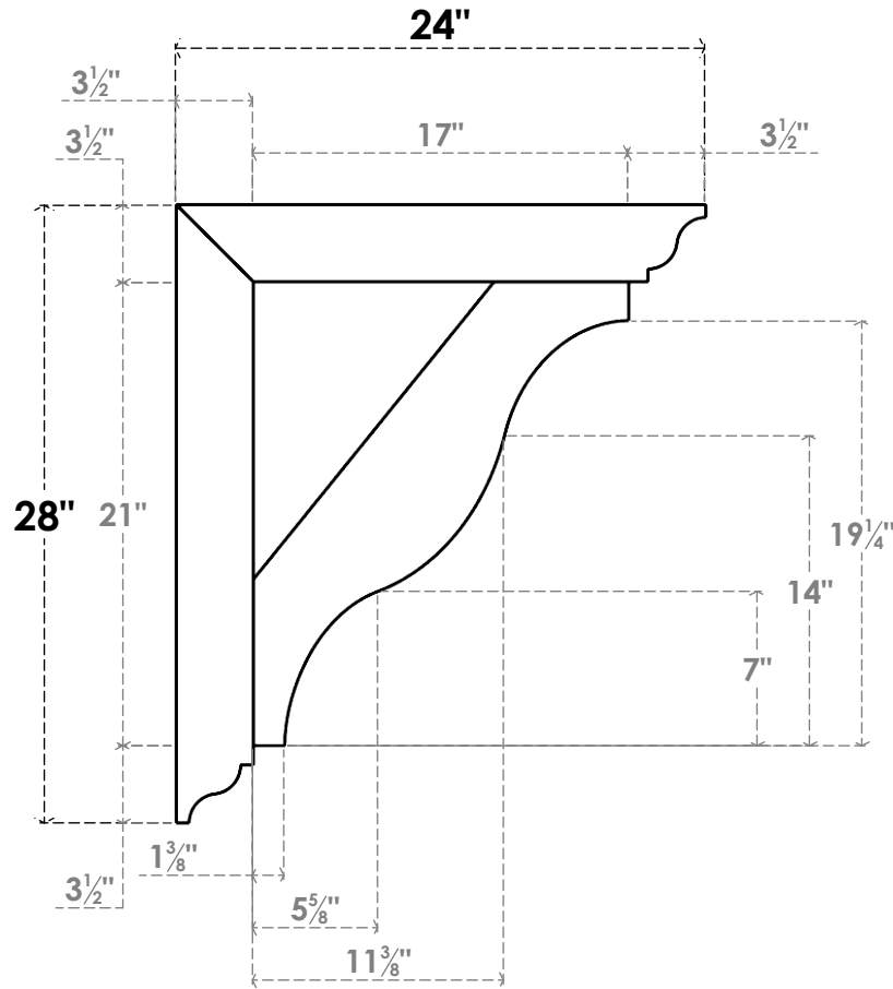
SIDE PROFILE
