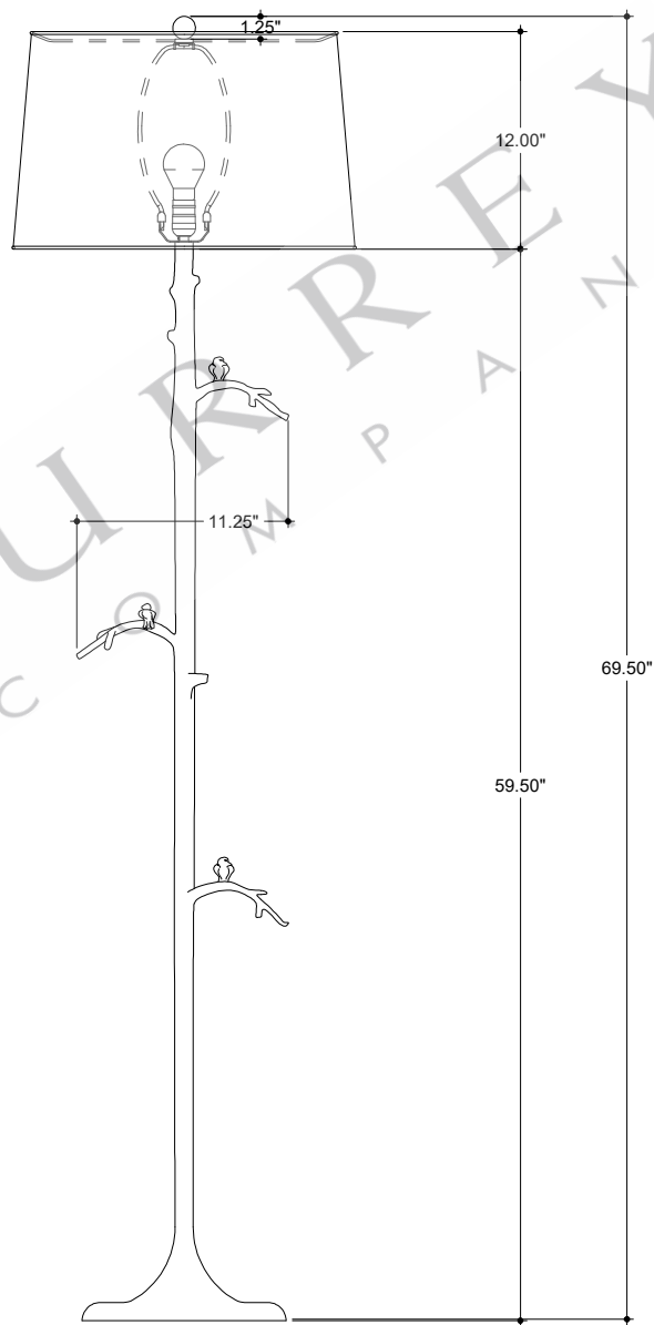
FRONT VIEW
