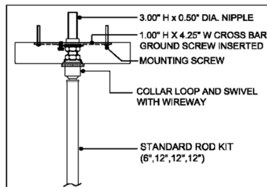
CANOPY DETAIL
