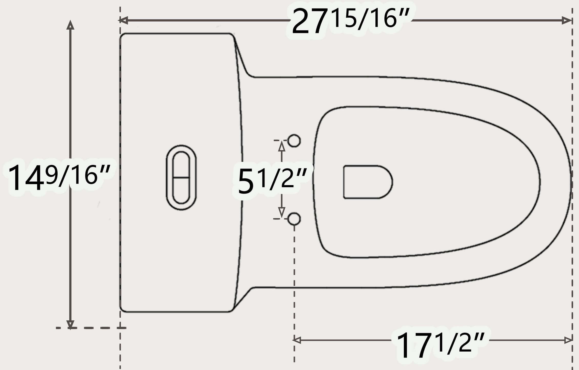
TOP VIEW
