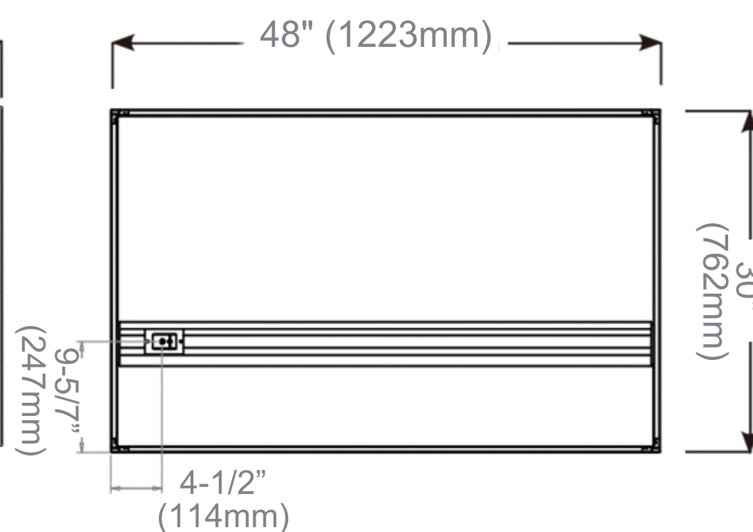
Back of Cabinet - Wire Access Location
