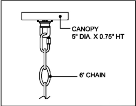
CANOPY DETAIL
