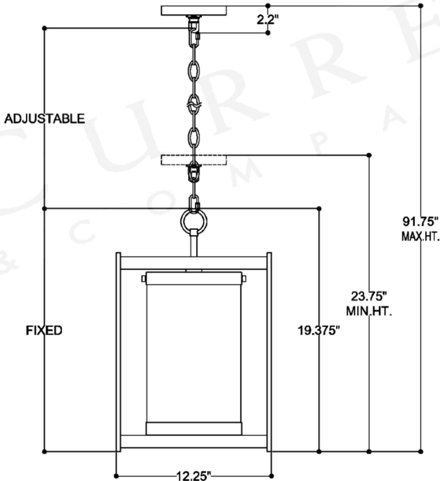
FRONT VIEW
